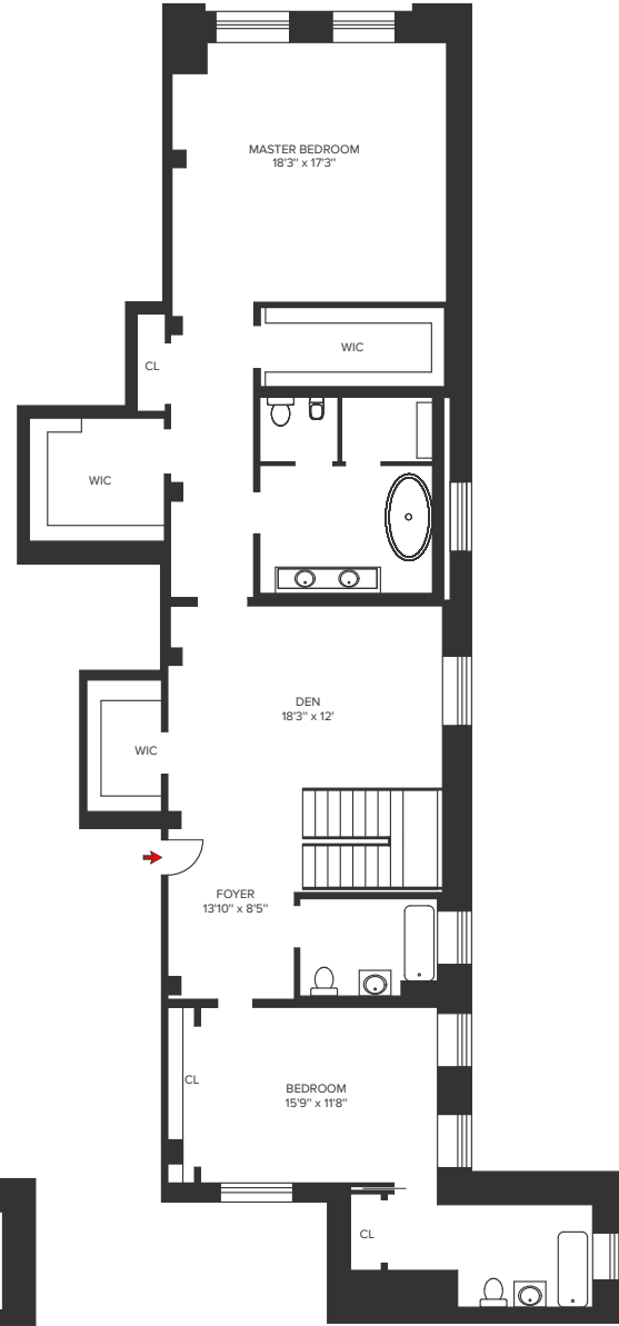
THIRD FLOOR
